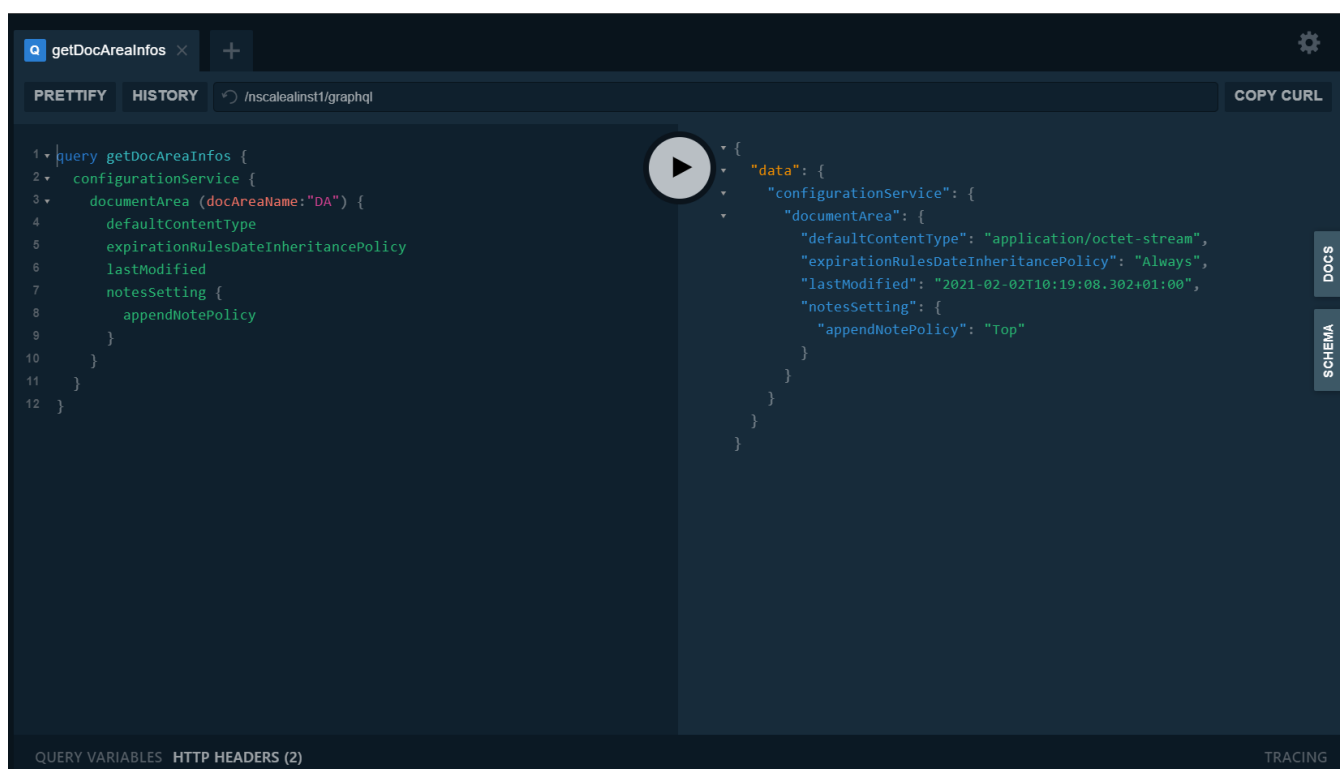
Figure 6. GraphQL query to get document area settings
